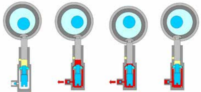
Function of the pump element
