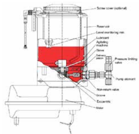
Function of the pump element
